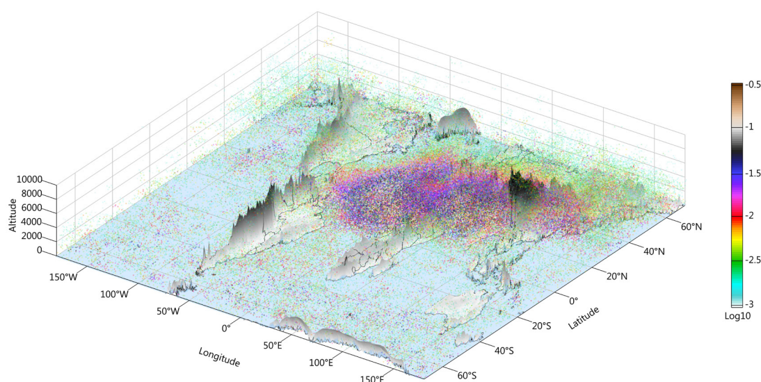
Figure 3. CALIOP-derived global three-dimensional particles map of the dust extinction coefficient (DEC) in the northern hemisphere spring of 2021. The colour scale is converted to log10 for improved visualization, corresponding to a minimum DEC of 0.001 and a maximum DEC of approximately 0.32.
