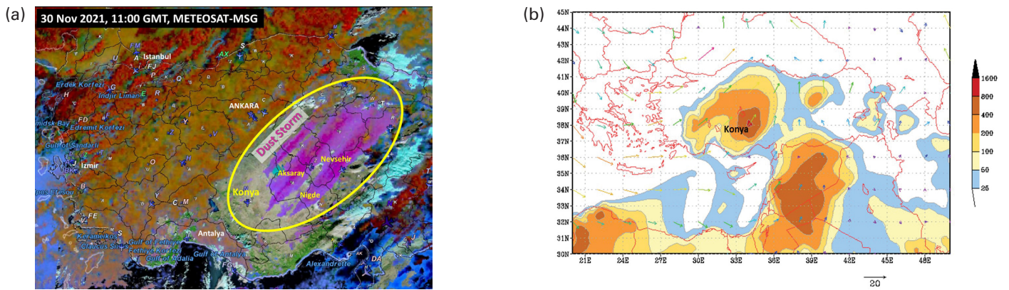
Figure 9. (a) RGB-Meteosat image: dust is represented by the colour pink within the encircled area ( Source: EUTMETSAT ); (b) Numerical output from the BSC-DREAMS8b model, showing forecast dust surface concentration for 30 November 2021 ( Source: Turkish State Meteorological Service )
